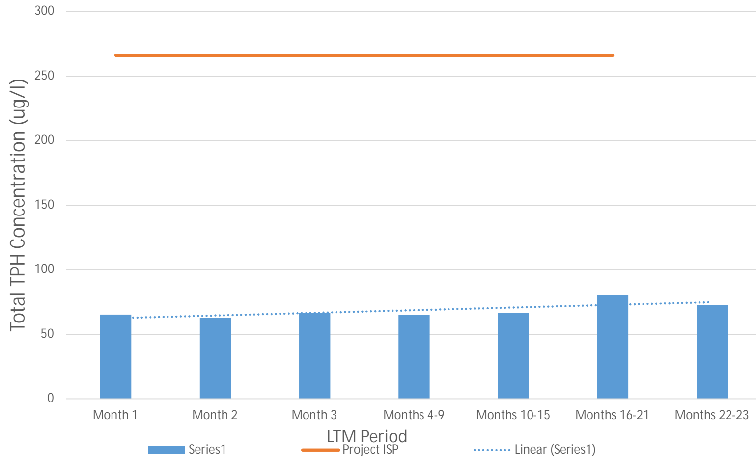
Average Total Petroleum Hydrocarbon Concentration by LTM Period March 2022 – February 2024
