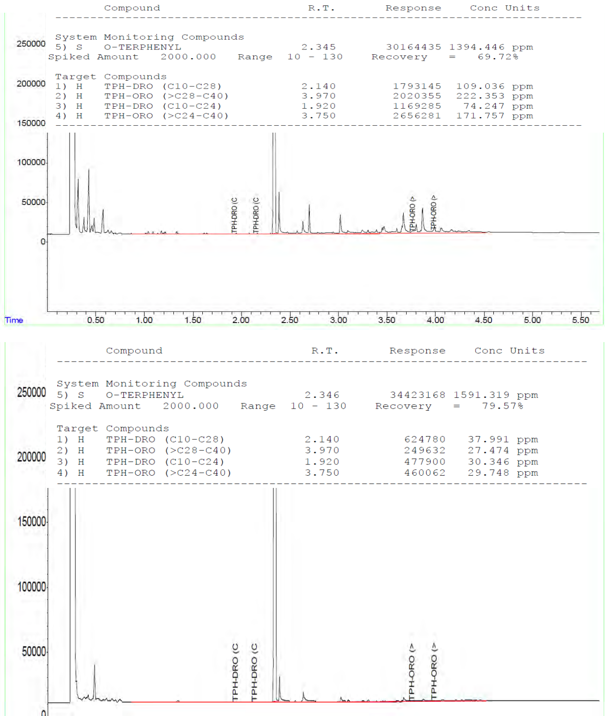
Figure D-10. 8015 TPH Chromatograms of Sample DA58265-9 (Top) and the Respective Method Blank (Bottom)
